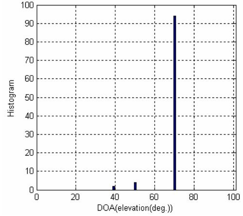
Fig.2: histogram of elevation angle for a single source located at (70^\circ, 40^\circ) , SNR = 10 dB by the proposed method with 5 elements on the z axes subarray
