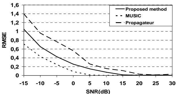
Fig.9. RMSE for a single source located at (90^\circ, 70^\circ) with a 2-Lshape array antenna versus SNRs
