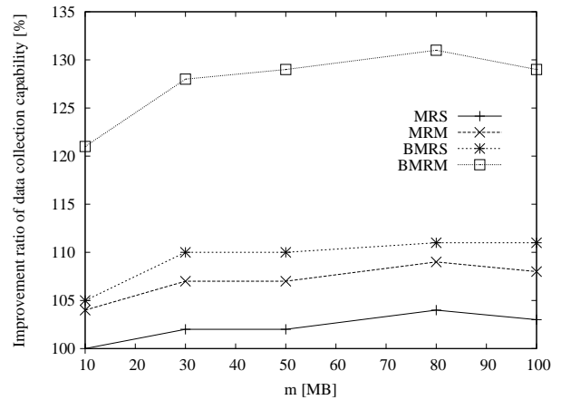
(c) For 30 source nodes.
