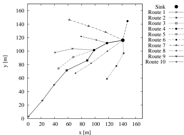
(b) The configuration obtained by MRM.
