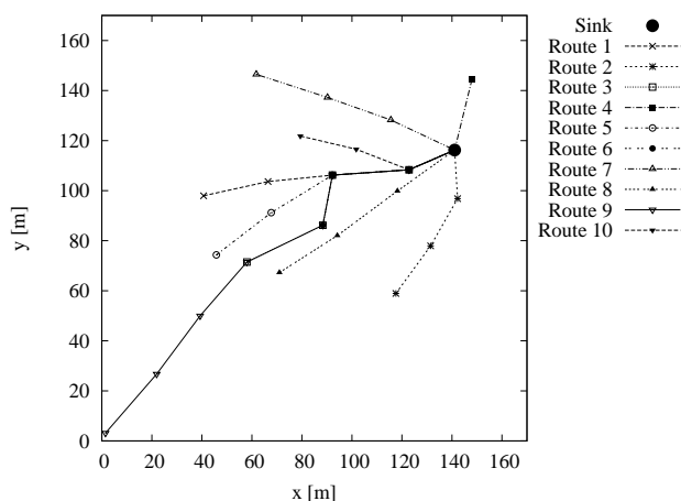
(a) The configuration obtained by MRS.
