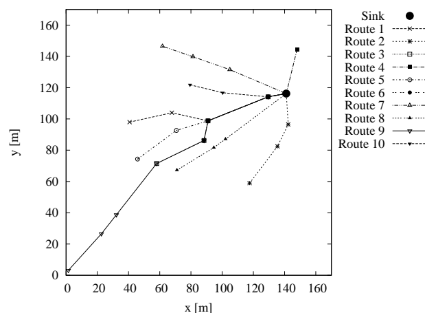
(b) The configuration obtained by BMRM.
