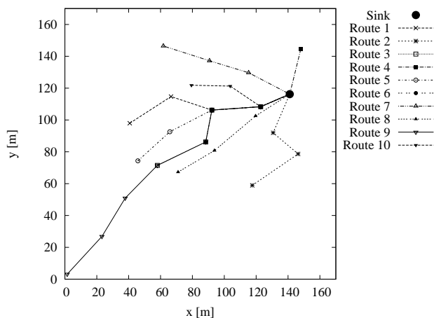
Fig. 4. An initial configuration.
