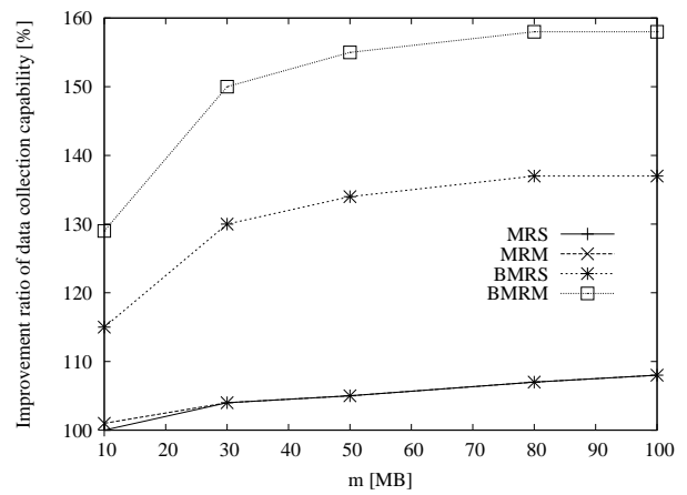
(a) For 10 source nodes.
