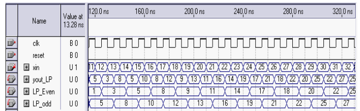
Fig.8. Low pass filter output
