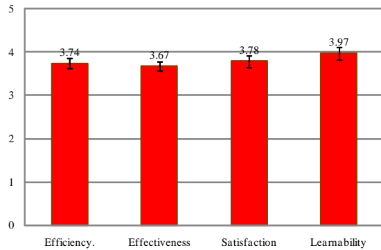
Figure 7: Evaluation on Results of Usability Testing.
