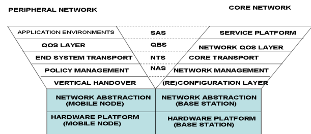
Figure 1: The complete architecture of Y-Comm
