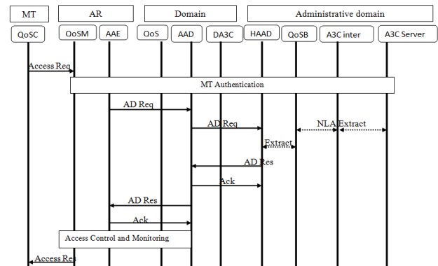
Figure 8: The Registration process
