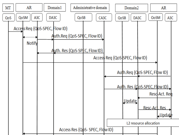
Figure 9: Connection initiation
