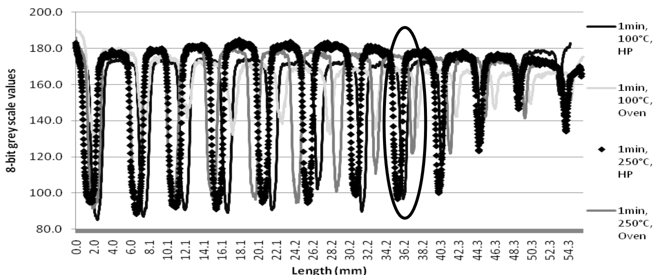
Fig. 4: Comparison between the melting effectiveness of oven and hot plate (HP)
