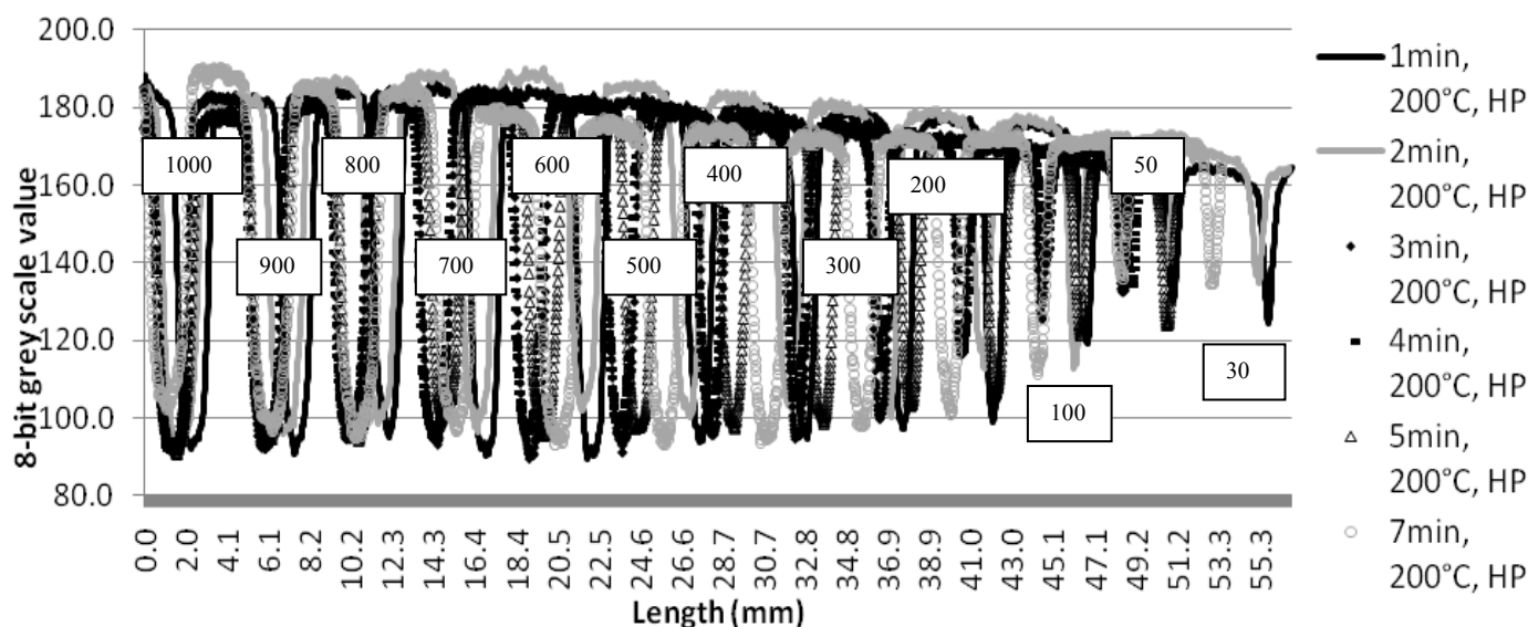
Fig. 7: Effect of melting time on melting effectiveness (text boxes indicate the line width ( \mu\text{m} ))
