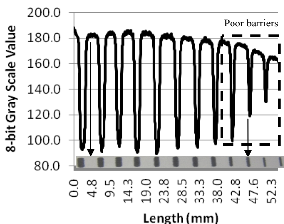
Fig. 2: Effect of line width on melting effectiveness
