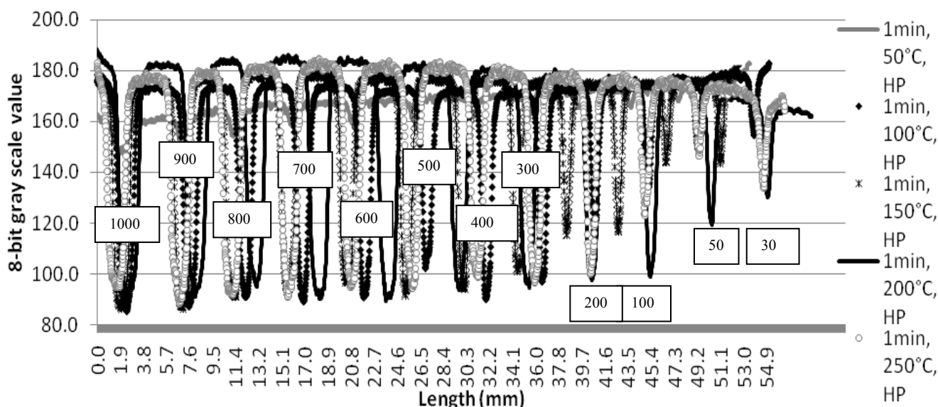
Fig. 6: Effect of temperature on melting effectiveness (text boxes indicate the line width ( \mu\text{m} ))
