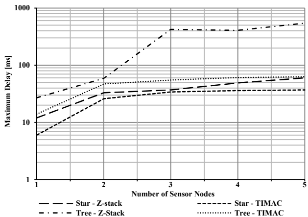
Fig. 6. Maximum delay as a function of the number of sensor nodes for both Z-Stack and TIMAC.
