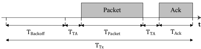
Fig. 1. Times associated to the 802.15.4 unslotted CSMA-CA algorithm.
