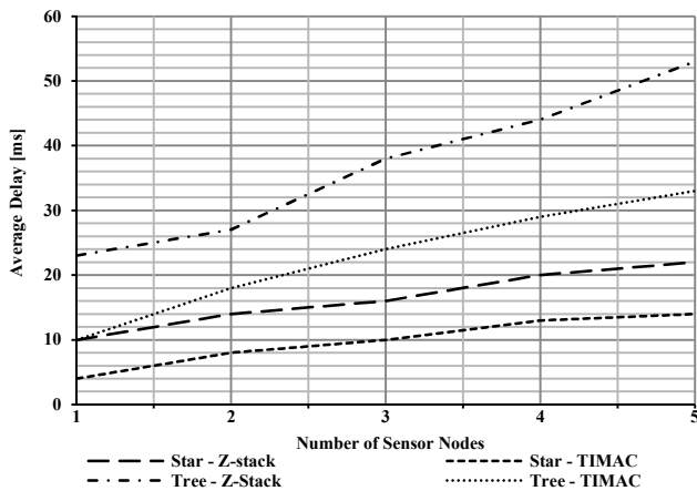
Fig. 5. Average delay as a function of the number of sensor nodes for both Z-Stack and TIMAC.
