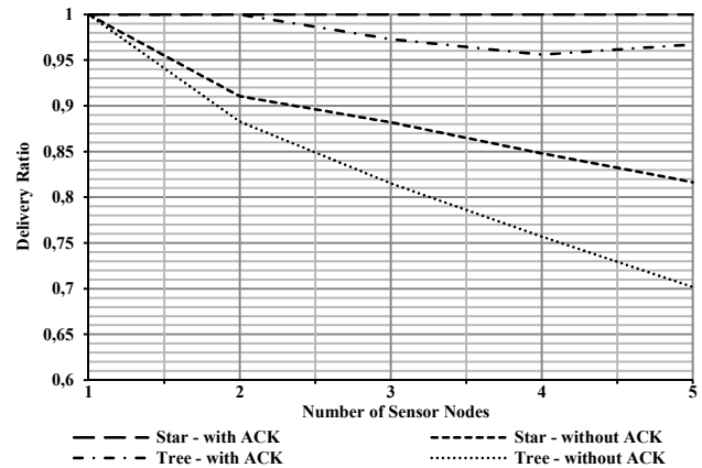
Fig. 3. DR measured with Z-Stack as a function of the number of nodes.
