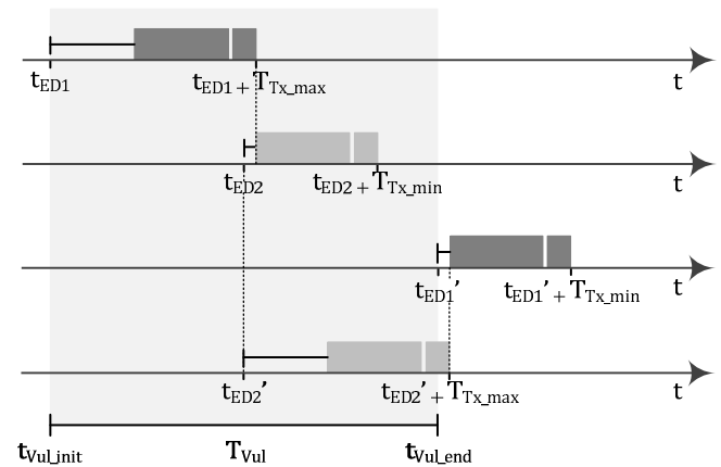
Fig. 2. Vulnerability window for the clock drift evaluation scenario.
