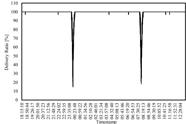
Fig. 7. DR with clock drift in a star topology with two hidden nodes.
