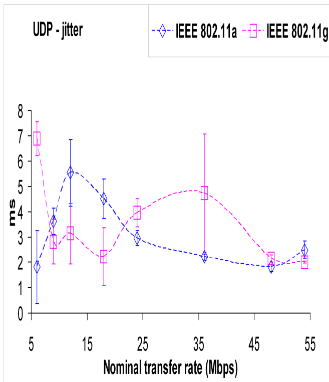
Fig. 7- UDP – jitter results versus technology and nominal transfer rate. Open PTMP.
