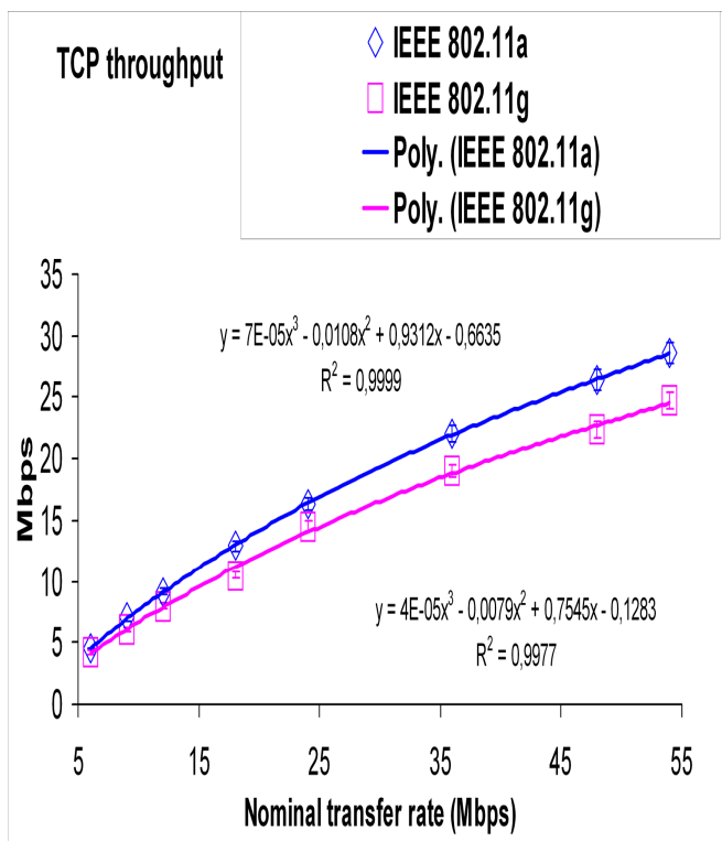
Fig. 4- TCP throughput (y) versus technology and nominal transfer rate (x). WPA2 PTP [12].
