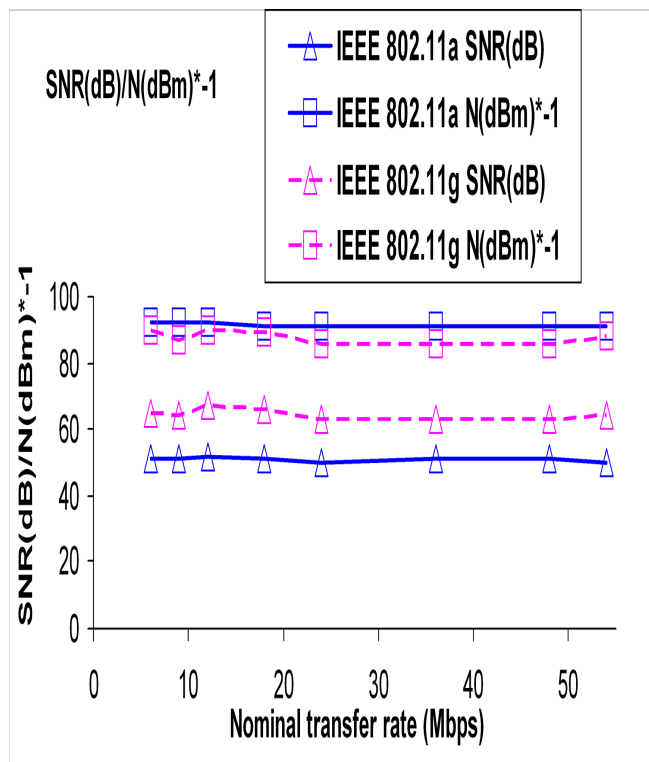
Fig. 2- Typical SNR (dB) and N (dBm). WPA2.
