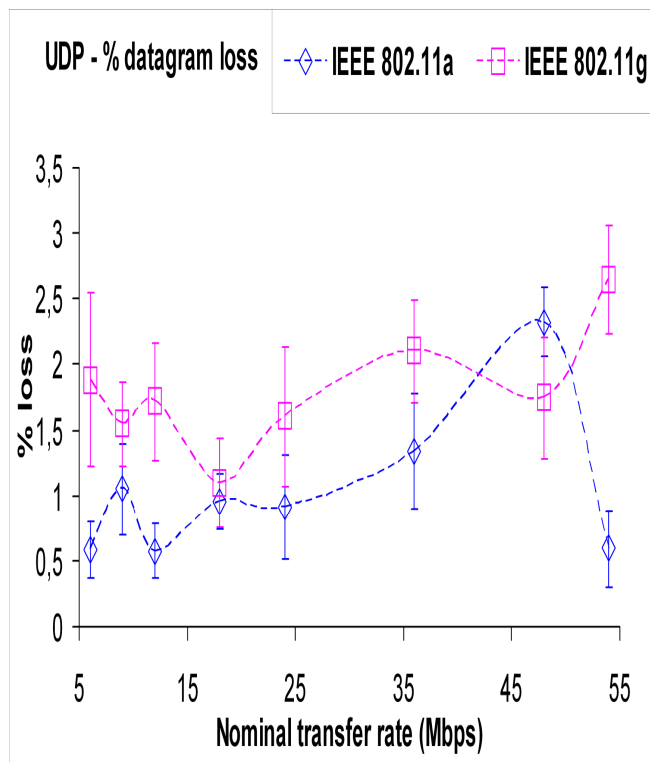
Fig. 9- UDP – percentage datagram loss results versus technology and nominal transfer rate. Open PTMP.
