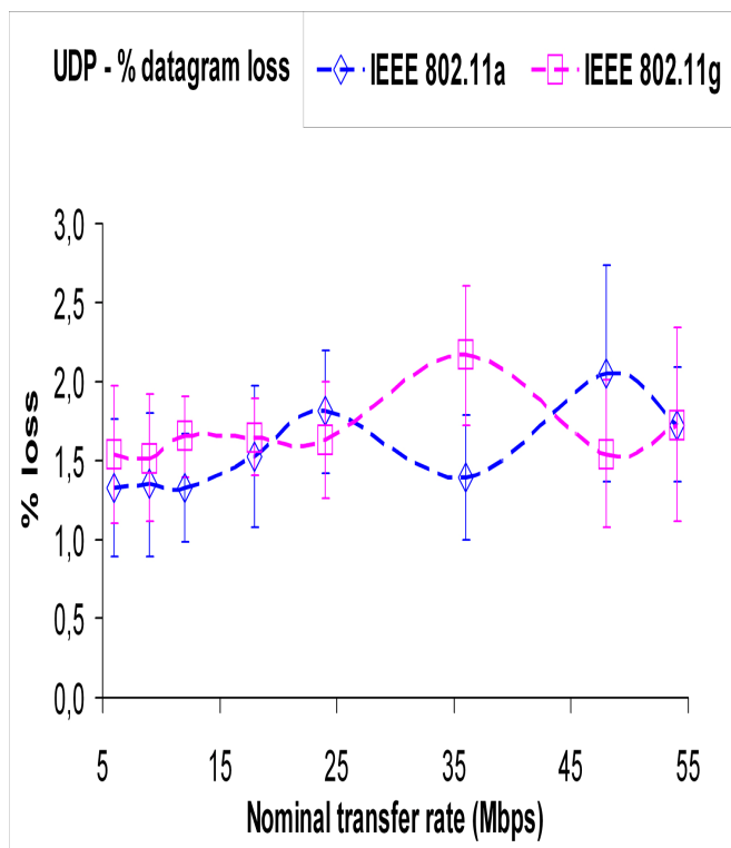
Fig. 8- UDP – percentage datagram loss results versus technology and nominal transfer rate. WPA2 PTMP.
