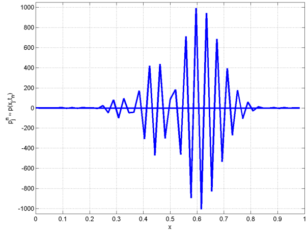
Fig. 1. Instability for N = 100 , \mu = 27 and x_\infty = 1 .
