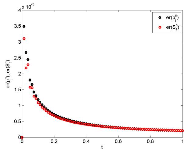
Fig. 2. Numerical estimated errors e_r(p^n) and e_r(S_f^n) versus t_n .
