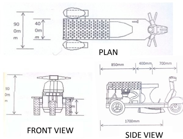
Fig 3. Different Technical Views of the Machine
