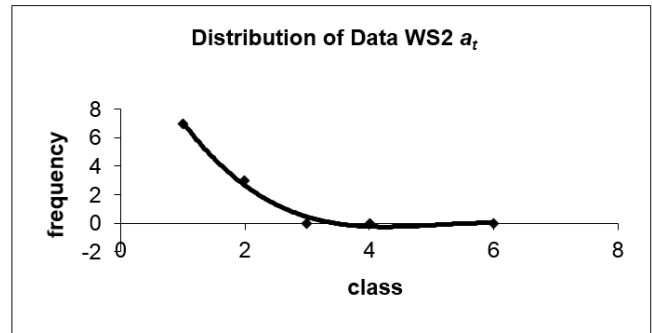
Fig. 5. Distribution of pallets' endurite moldings flow times at Workstation 2 (WS2): Approximated to exponential with a mean of 23.03 seconds
