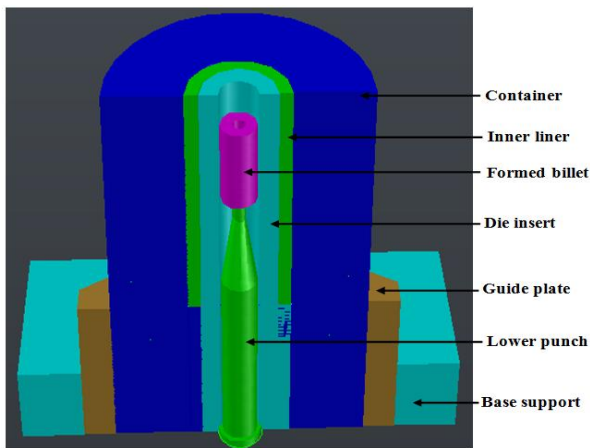
Fig.1. Double cup extrusion tooling setup
