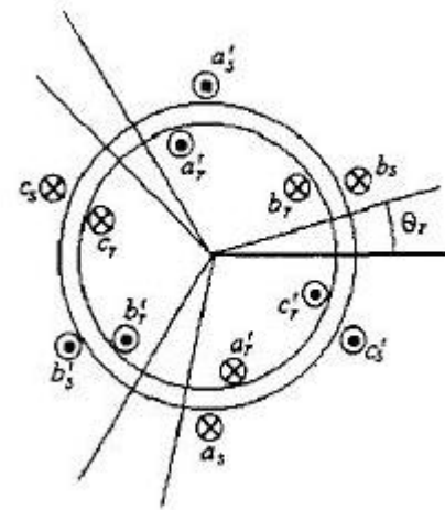
Fig. 3. Schematic image of three phase induction motor
