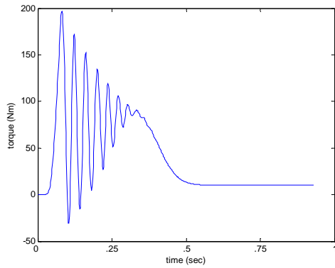
Fig. 5. 50hp induction motors torque under sinusoidal supply condition
