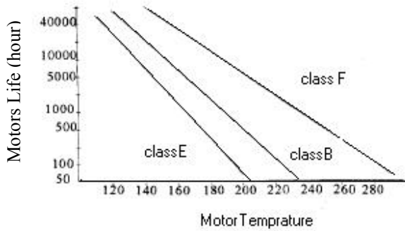
Fig. 1. Induction motors temperature and its life relation in three different classes
