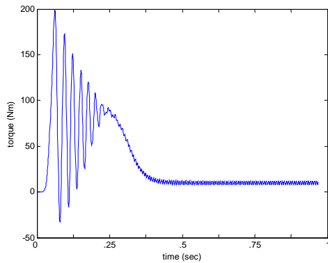
Fig. 7. 50hp induction motors torque under non ideal supply condition
