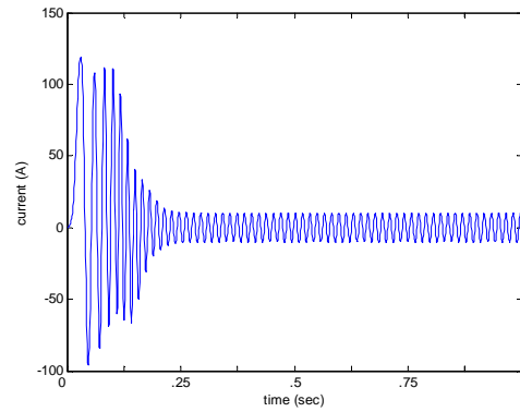
Fig. 2. Current of one phase of induction motor
