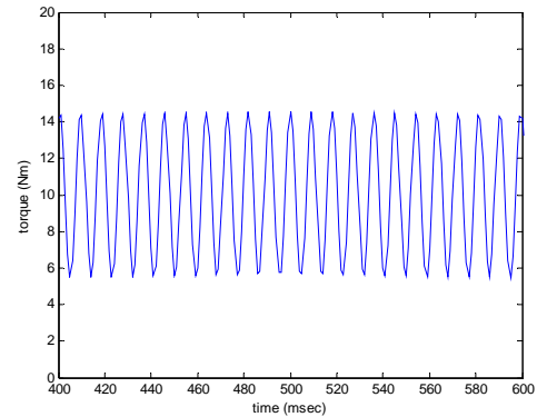
Fig.5. 50hp induction motors torque oscillations in steady state under non ideal supply condition
