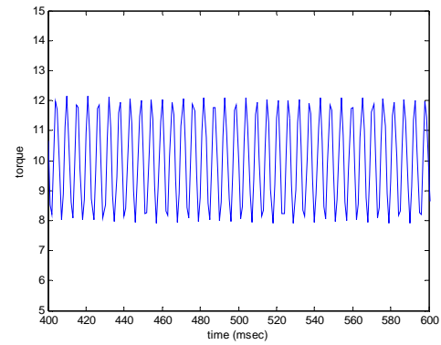
Fig.5. 3hp induction motors torques oscillations in steady state under non ideal supply condition
