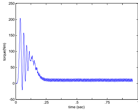
Fig. 6. 3hp induction motors torque under non ideal supply condition
