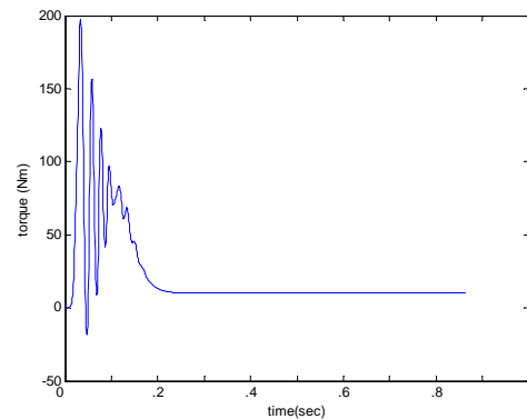
Fig. 4. 3hp induction motors torque under sinusoidal supply condition
