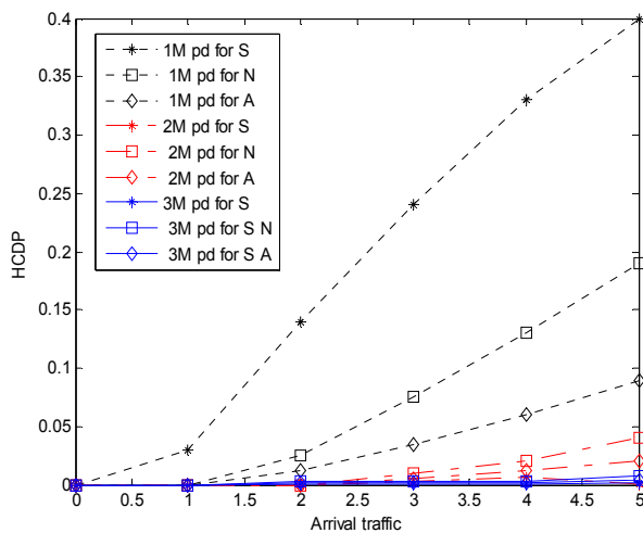
Fig. 5. HCDP (Pd) for class-1 calls with 1M: 2M: 3M = 25:50:25
