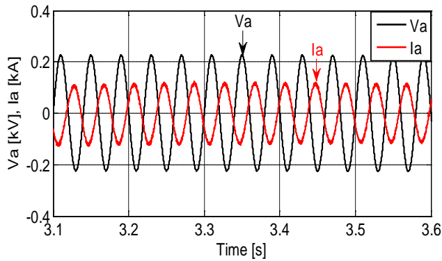
Fig. 7. Primary voltage and current at unity power factor.
