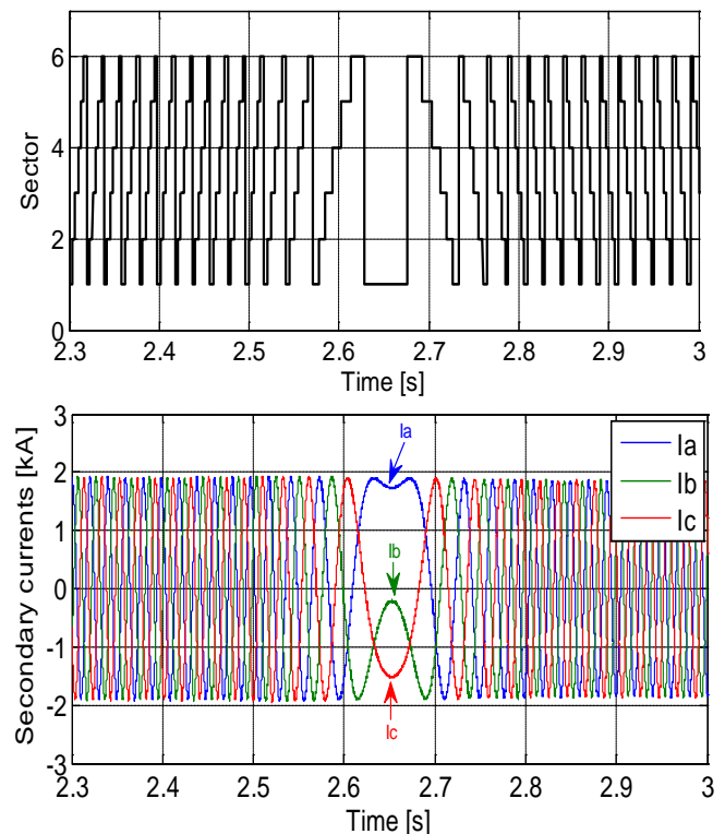
Fig. 6. BDFRG secondary voltage positions and secondary current waveforms showing a phase sequence reversal during the speed mode transition at unity power factor.
