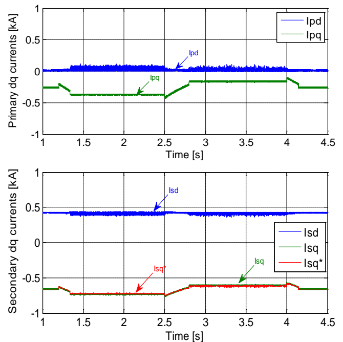
Fig. 5. MPF responses of the BDFRG current components in the corresponding rotating reference frames.
