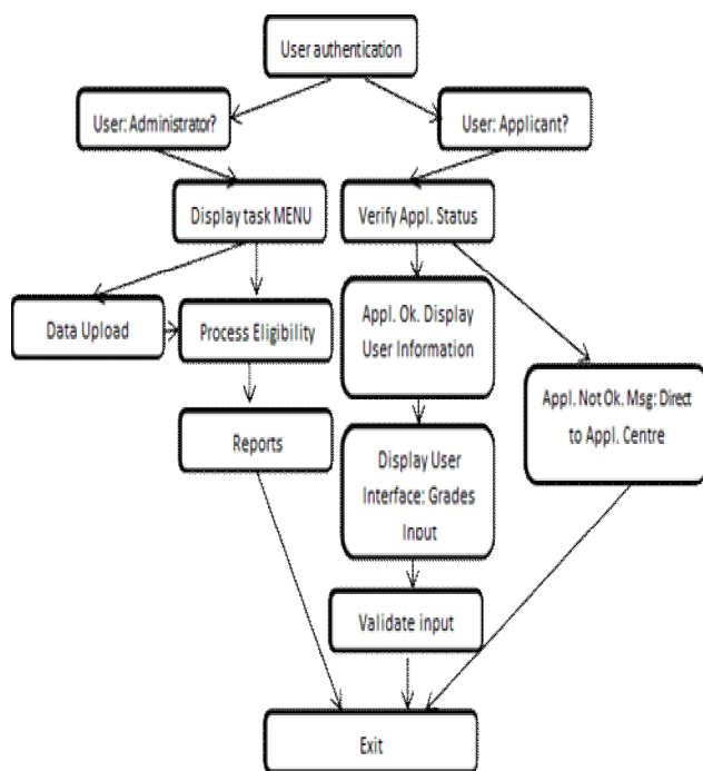
Fig. 4. Data Flow Architecture
