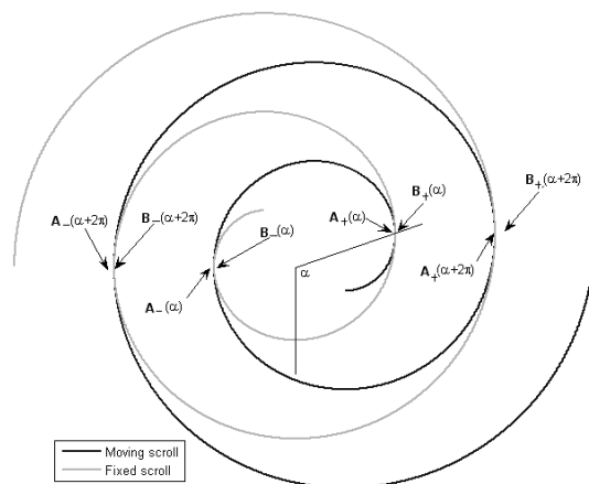
Figure 5. Illustration of the areas bounded by the fixed and moving scrolls
