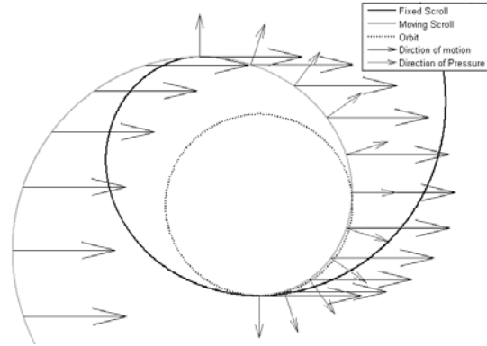
Fig. 6 Relationship between the direction of motion and the direction of the sum of the pressure
