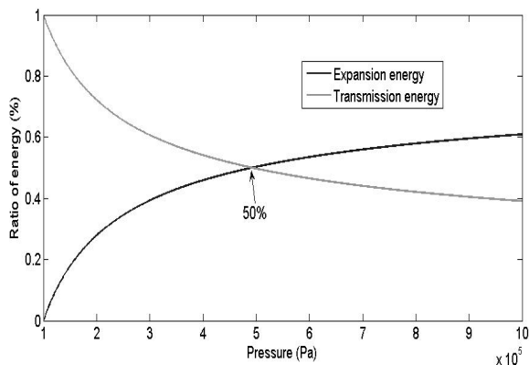
Fig. 8 Composition of air energy
