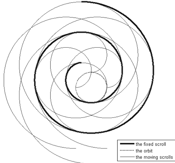
Fig. 4. A family of spirals
