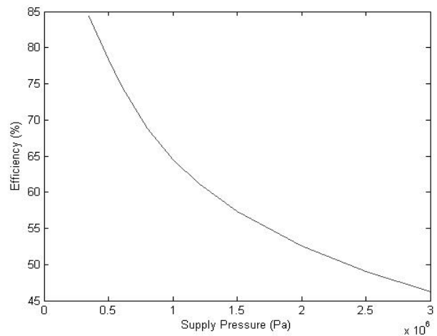
Fig. 9 Energy efficiency vs. supply pressure
