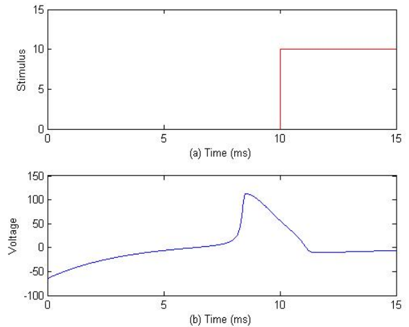
Fig.1: The voltage trace v_s generated by a small step-current I_s . This small trace of neural voltage is sufficient to retrieve the maximal conductances.
