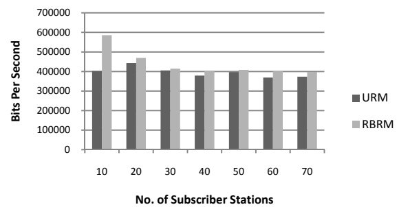
Fig. 6. Total throughput for rtPS
