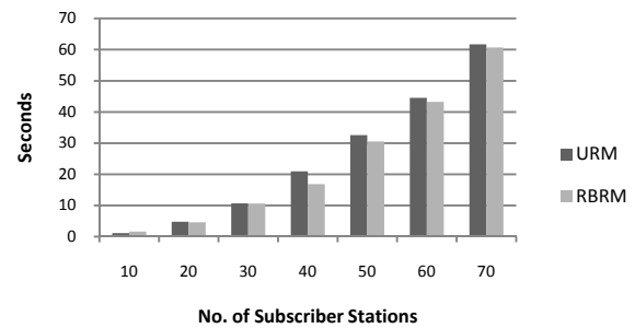
Fig. 7. Total end-to-end delay for rtPS
