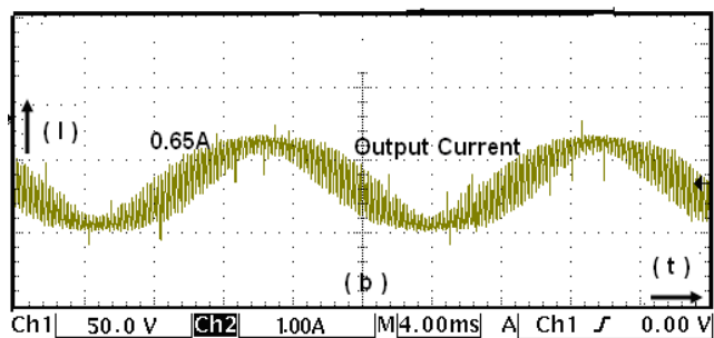
Fig. 8. Load Current during experiment
