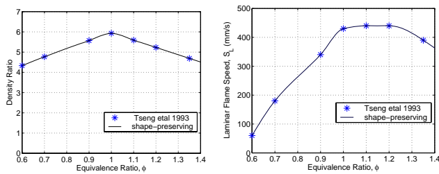
Fig.1 Density ratio and laminar flame speed for CH 4
