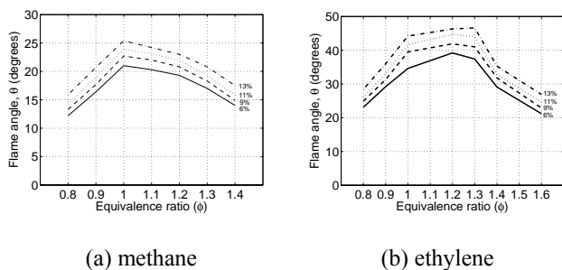
Fig.5 Flame angle for different fuel/air mixtures
