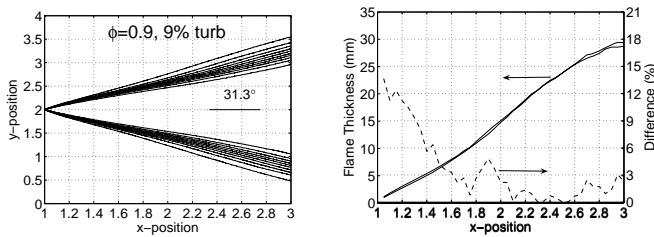
Fig.4 Flame zone, flame angle and flame thickness for C_2H_4
