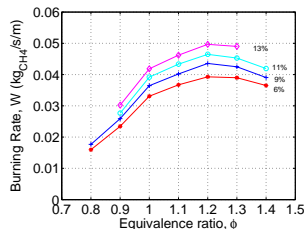
Fig.7 Mean burning rate of methane
