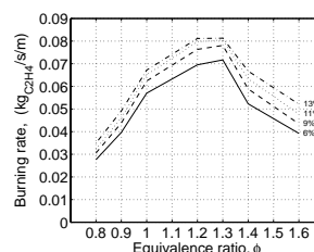
Fig.10 Mean burning rate of ethylene
