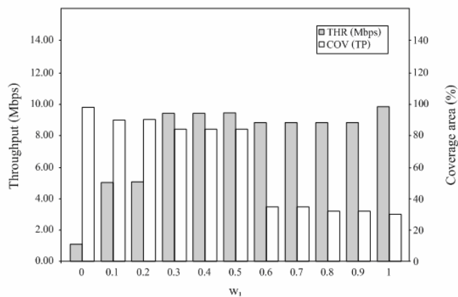
Fig.3 System throughput and coverage of WLANs using 6 APs
