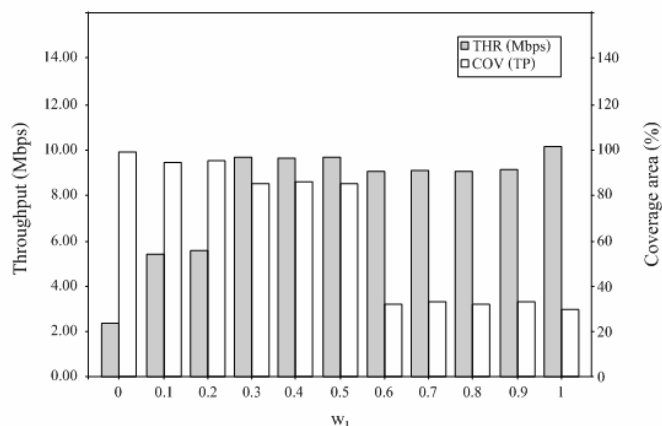
Fig.4 System throughput and coverage of WLANs using 7 APs
