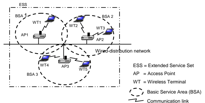
Fig.1 Infrastructure-based WLANs
