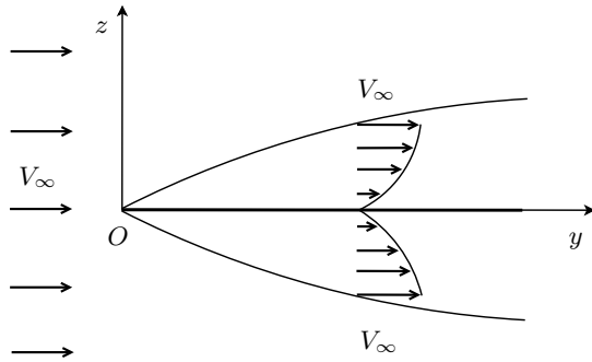
Figure 1: Boundary layer over a thin plate.
