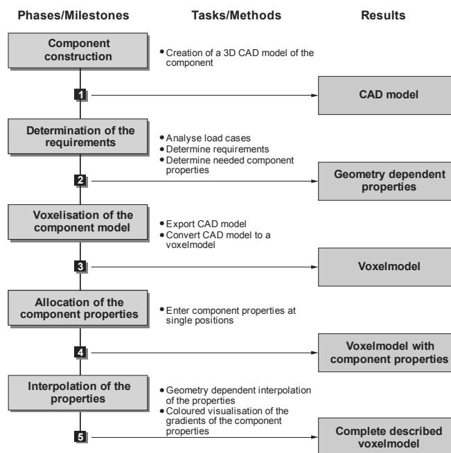
Fig. 2: Procedure model for the description of functional graded components
