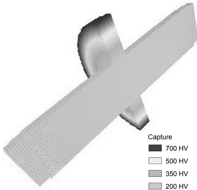
Fig. 5: Voxelmodel of the cut flange steel shaft with visualisation of the hardness gradient included
