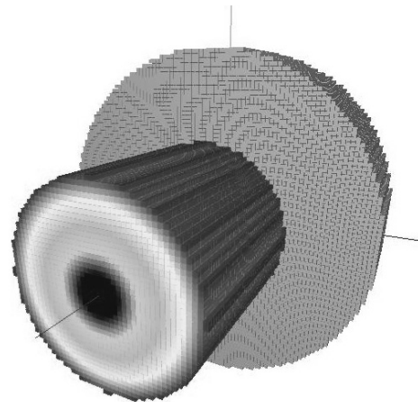
Fig. 4: Voxelmodel with interpolated characteristic gradient in the stub shaft.
