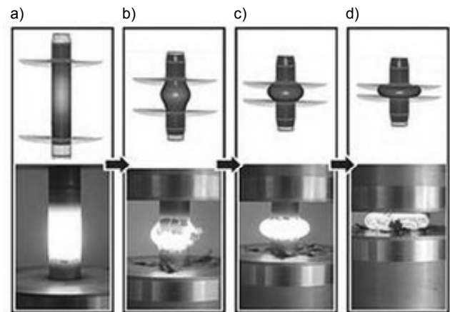
Fig. 1: Transforming process of the steel shaft (Prof. Steinhoff, University of Kassel)
