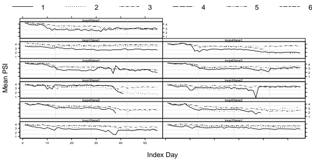
Fig. 4 Mean PSI for each subject (loop/lane) on different surface thickness versus index day
