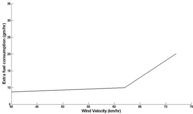
Fig. 8: Plot of extra fuel consumed due to overcooling with wind velocity at temperatures of -10^{\circ}\text{C} and 27^{\circ}\text{C} .
