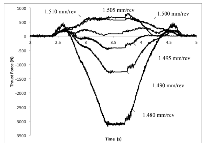
Fig 5. Axial force for tapping operation of AISI 1045 carbon steel at cutting speed of 30 m/min.
