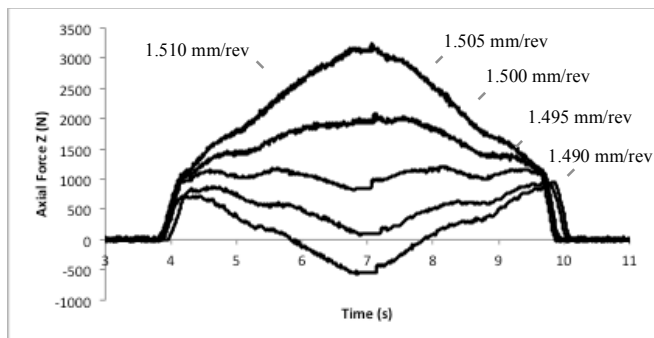
Fig 7. Axial force for thread forming operation at speed of 10 m/min.
