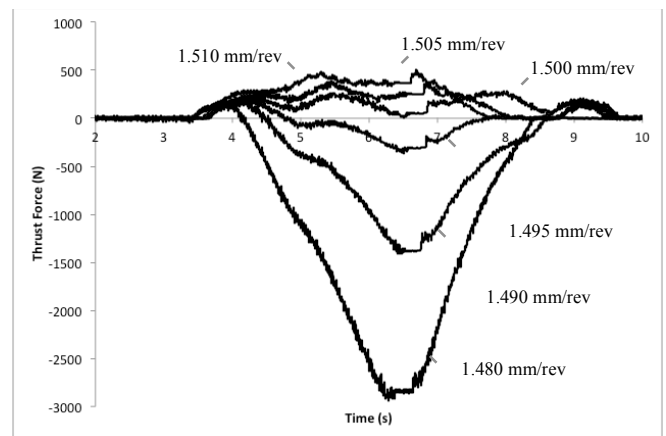
Fig 4. Axial force for tapping operation of AISI 1045 carbon steel at cutting speed of 10 m/min.
