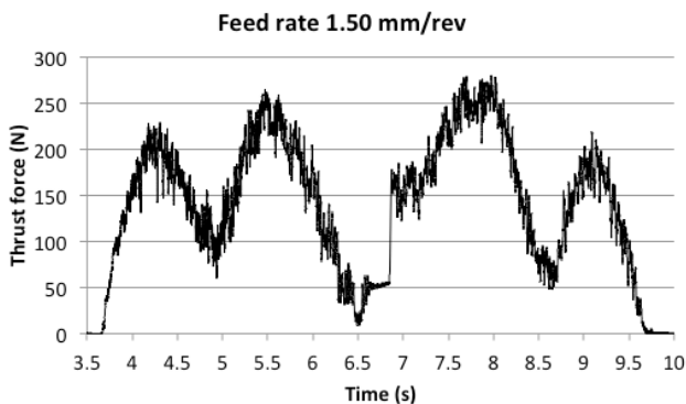
Fig 2. Thrust force during the tapping operation of AISI 1045 carbon steel at cutting speed of 10 m/min. Thread length is 16 mm with a feed rate of 1.500 mm/rev.
