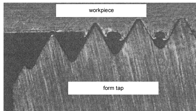
Fig 1. Thread forming operation and the split crest [6].
