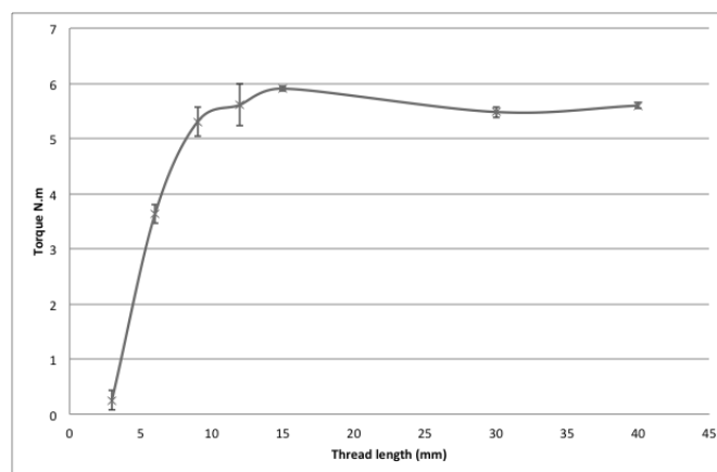
Fig 9. Effect of thread length on the mean torque signal for tapping operation at cutting speed of 10 m/min.
