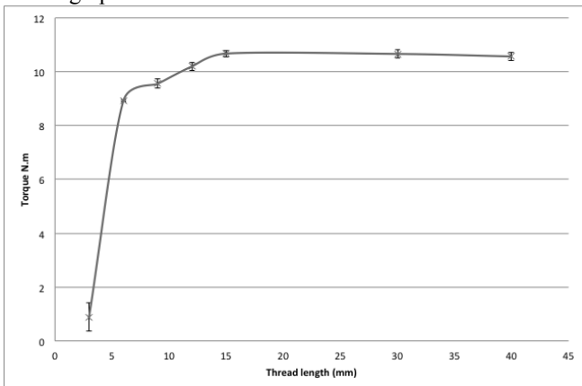
Fig 11 Effect of thread length on the mean torque signal for forming operation of AISI 1045 carbon steel at speed of 10 m/min.
