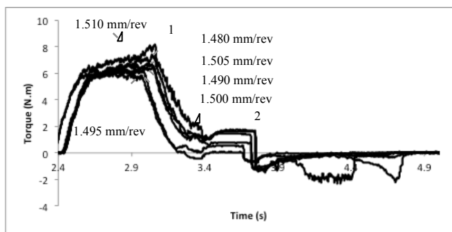
Fig 6. Torque signal for tapping operation of AISI 1045 carbon steel at cutting speed of 30 m/min.
