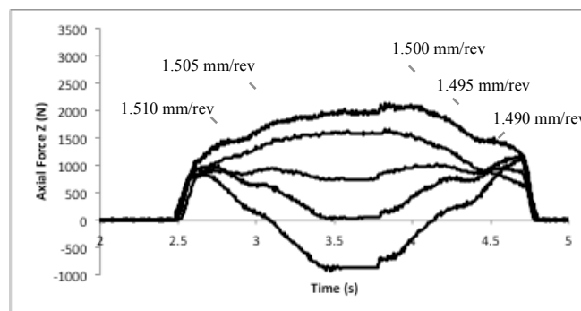
Fig 8. Axial force for thread forming operation at speed of 30 m/min.
