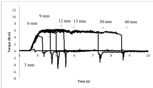
Fig 10. Torque signal for different thread lengths when tapping at cutting speed of 10 m/min.
