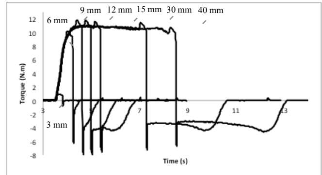
Fig 12. Torque signal for different thread lengths for the forming operation at speed of 10 m/min.
