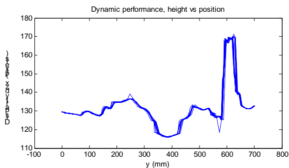
Figure 13. Result of 10 test runs on sugar beet with weed on uneven ground.
