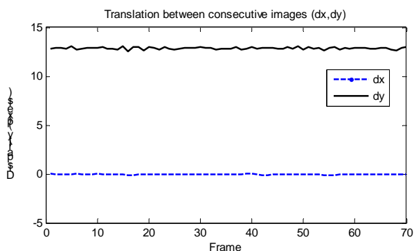
Figure 10. Translation d_x , d_y on reference track 1.
