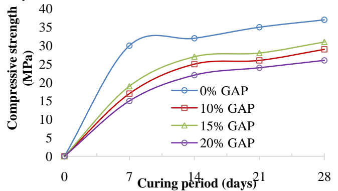
Fig. 4. Compressive strength development over time of tested plasters produced from GAP waste powder
