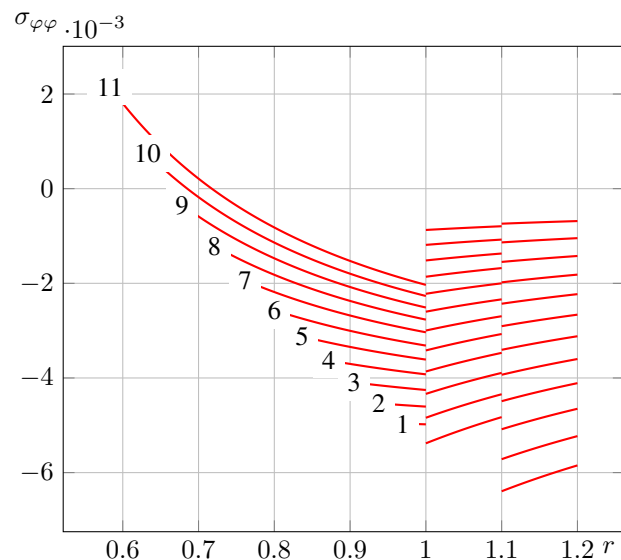
Fig. 3. Circumferential stress \sigma_{\varphi\varphi} in the growth cylinder at different times. Line denoted by number i corresponds to the growth time t_i .
