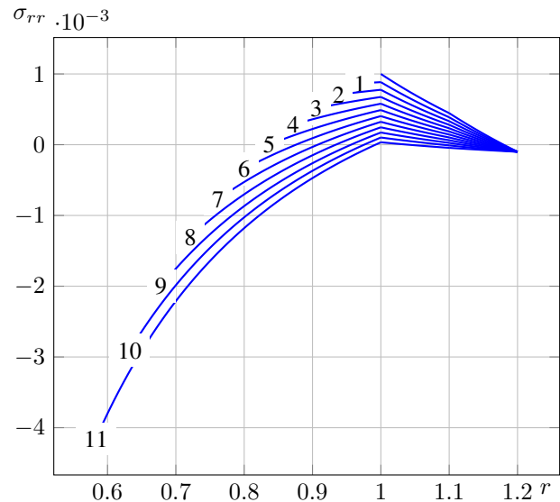
Fig. 2. Radial stress \sigma_{rr} in the growth cylinder at different times. Line denoted by number i corresponds to the growth time t_i .
