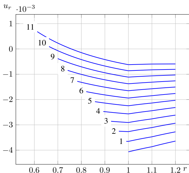
Fig. 4. Radial displacement u in the growth cylinder at different times. Line denoted by number i corresponds to the growth time t_i .
